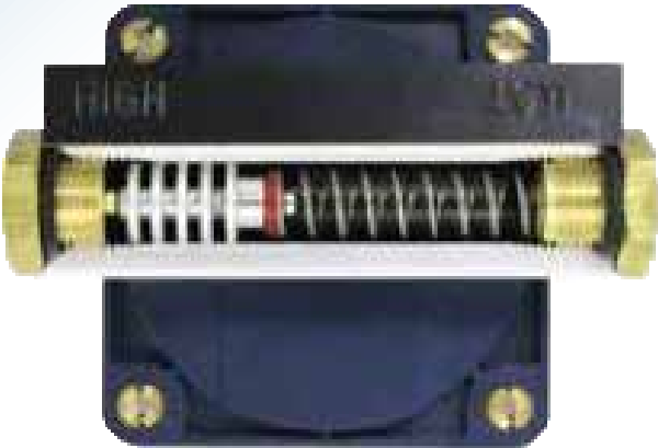
Fig. 4 Operating principle
