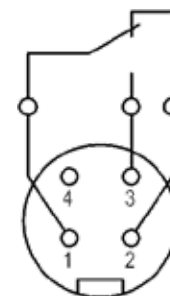
Fig. 1. Reed contact connection
